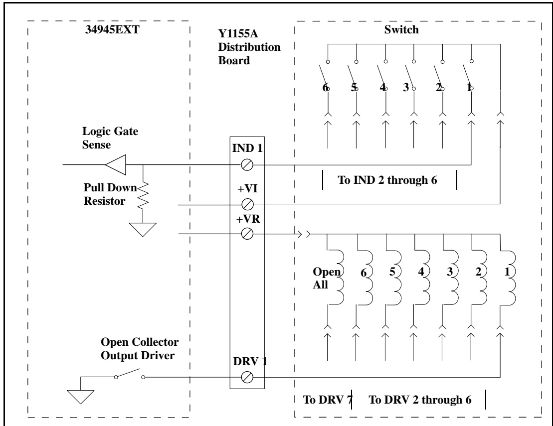
Figure 5-3. Single-Coil Switch Connection Diagram (separate position indicators).
